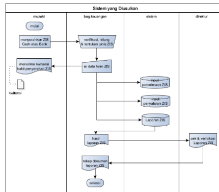
Gambar 2. Flowchart sistem usulan
