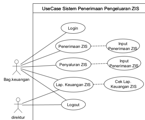
Gambar 3. Usecase diagram system
