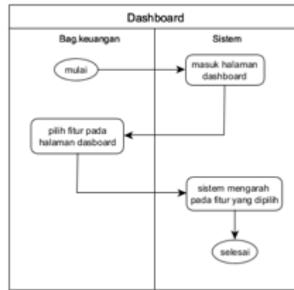
Gambar 5. Activity diagram Dashboard
