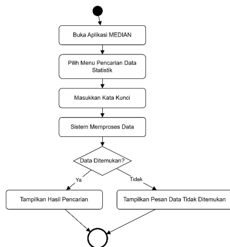
Gambar 2. Activity Diagram Pencarian Data Statistik
