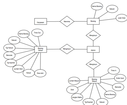
Gambar 3. 6 Entity Relationship Diagram.
